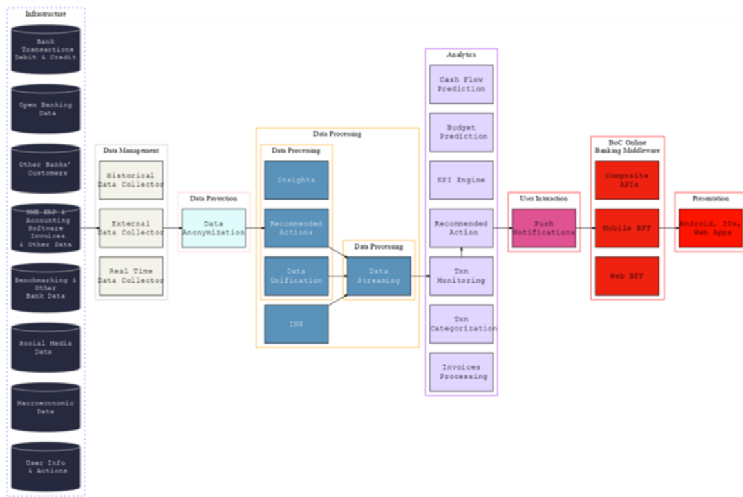
Figure 47 Business Financial Management pilot pipeline in-line with the IRA
