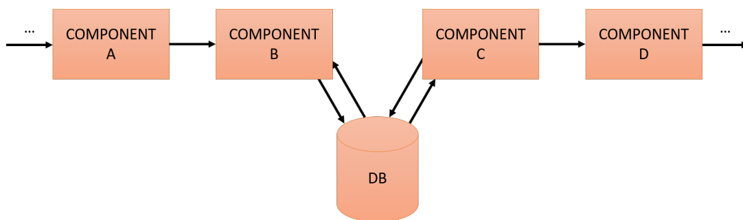
Figure 32 Communication through DB
