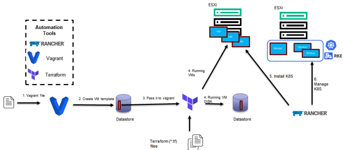
Figure 25 Automated K8S cluster creation with Rancher
