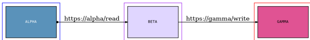
Figure 35 Cat Pipeline
