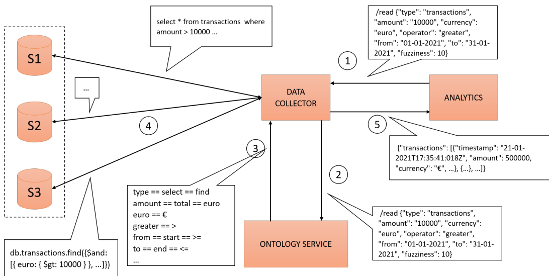
Figure 38 Ontology Services
