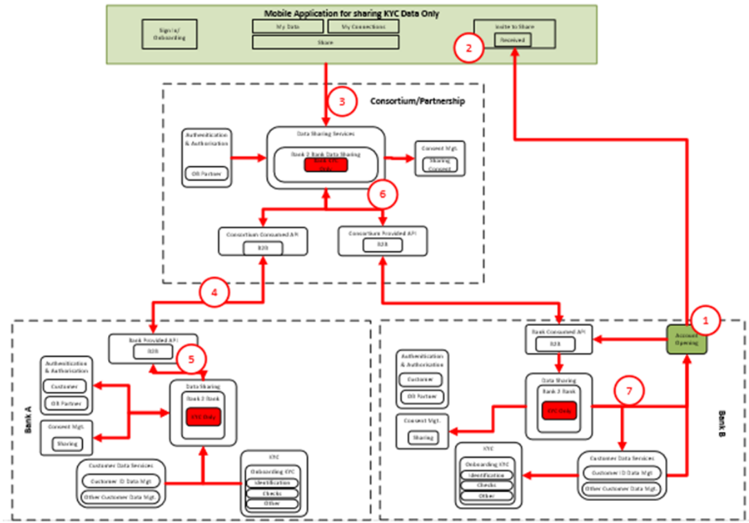
Figure 42 Customer-Centric Data Analytics pilot workflow - KYC Data Sharing Process - Technical Workflow
