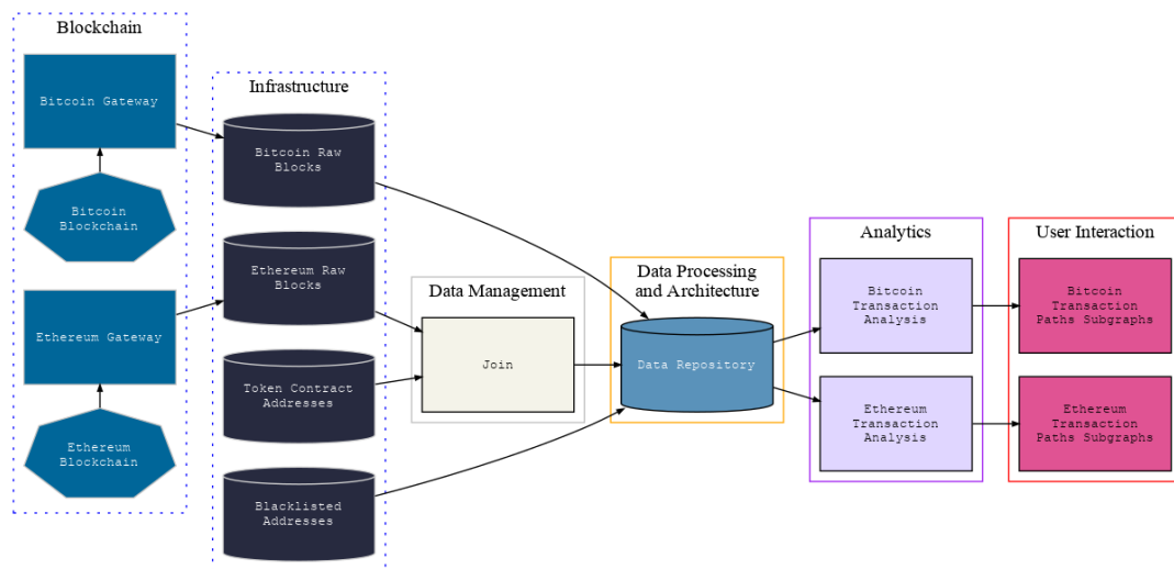
Figure 51 Blockchain Transaction Graphs Analysis pilot pipeline in-line with the IRA
