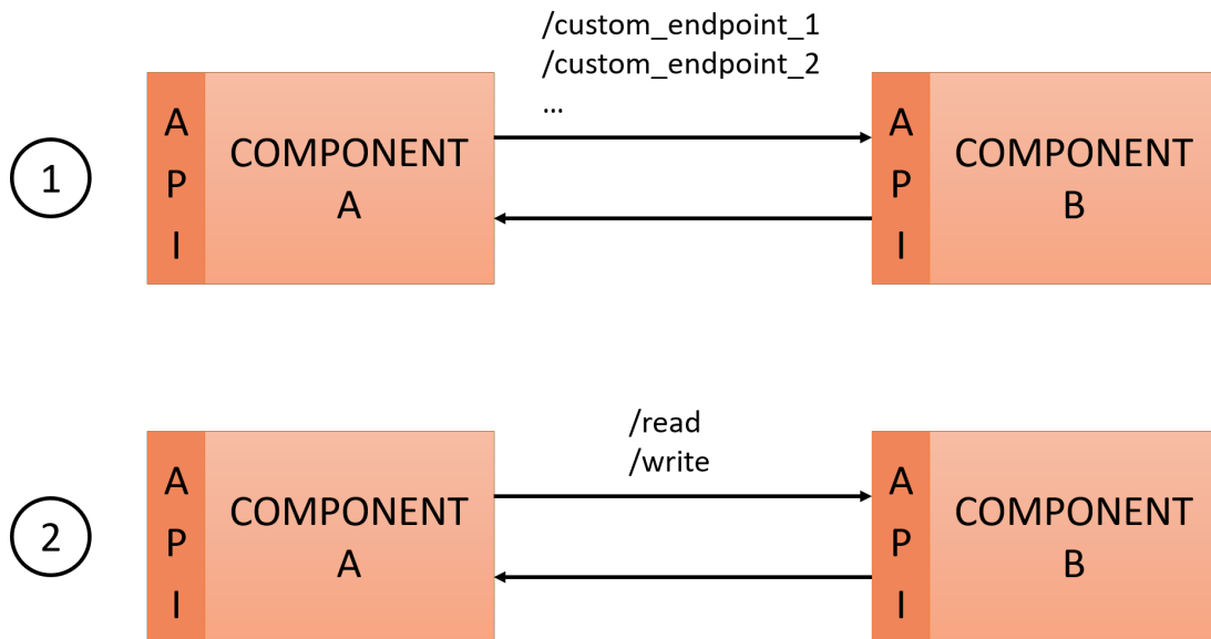
Figure 31 Component API
