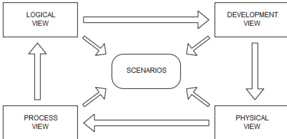
Figure 19 "4+1" views
