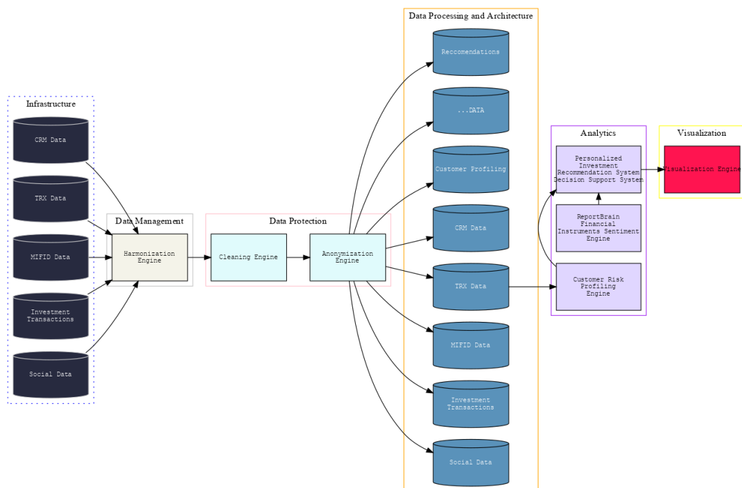
Figure 48 Personalized Closed-Loop Investment Portfolio Management pilot pipeline in-line with the IRA
