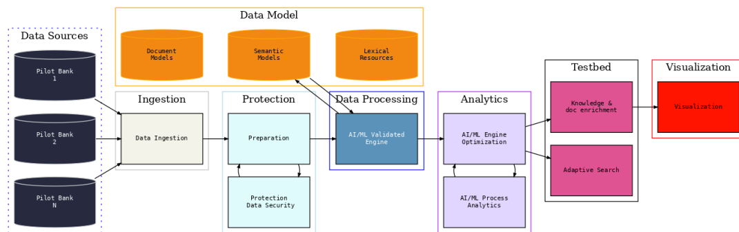
Figure 57 Open Inter-banking pilot pipeline in-line with the IRA
