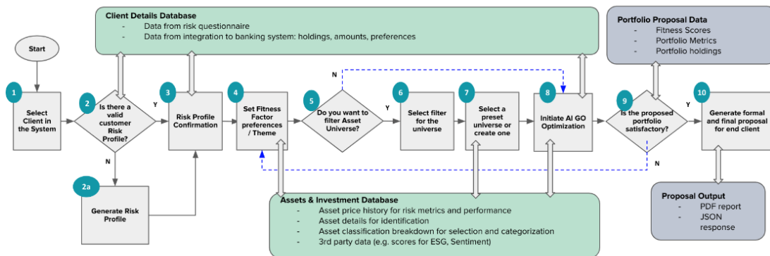
Figure 44 Personalized Portfolio Management pilot workflow
