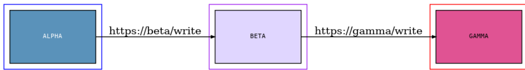
Figure 36 Classic Pipeline
