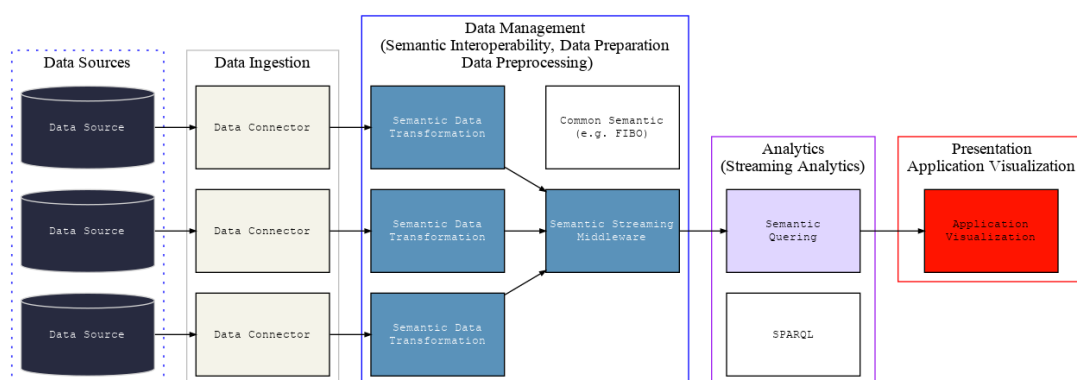
Figure 28 Pipeline for a Scenario involving Semantic Interoperability Across Diverse Data Sources
