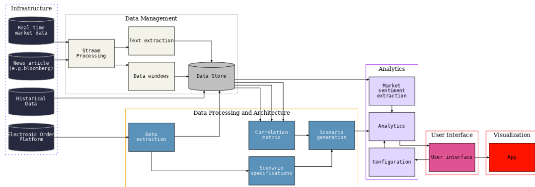
Figure 40 Real-Time Risk Assessment pilot pipeline in-line with the IRA
