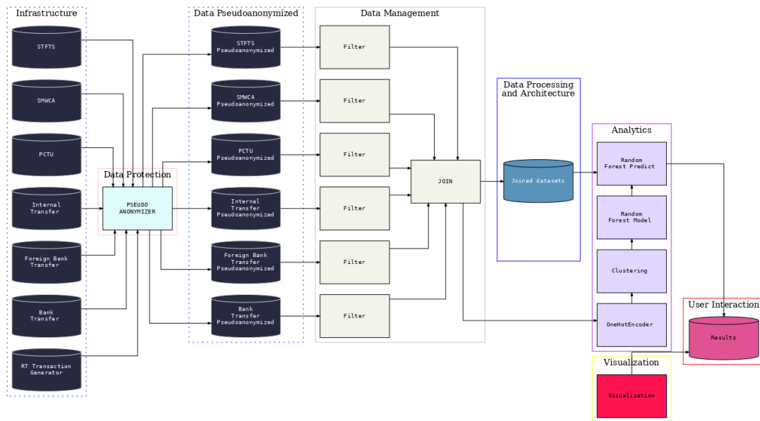
Figure 52 Real-time cybersecurity analytics pilots pipeline in-line with the IRA
