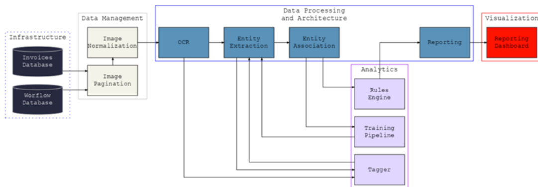
Figure 39 Invoices Processing pilot pipeline in-line with the IRA
