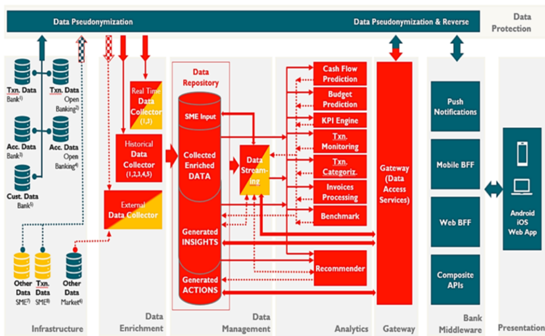
Figure 46 Business Financial Management pilot workflow
