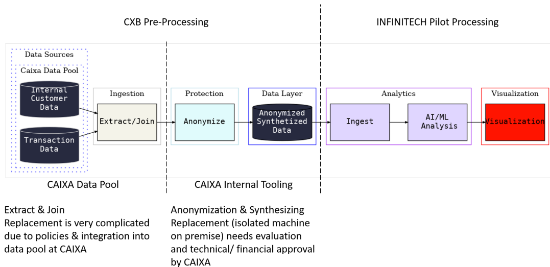
Figure 49 Financial Crime pilot pipeline in-line with the IRA
